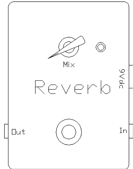
Diagram E: Reverb pedal
